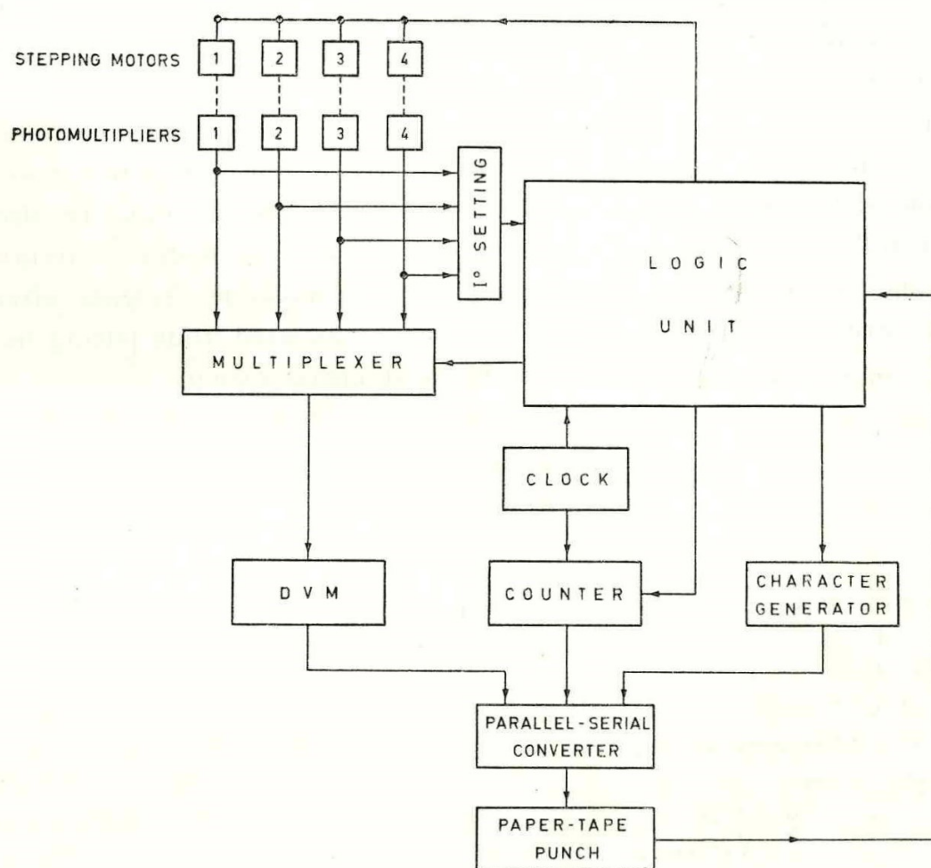
Fig. 3 — System block diagram.
